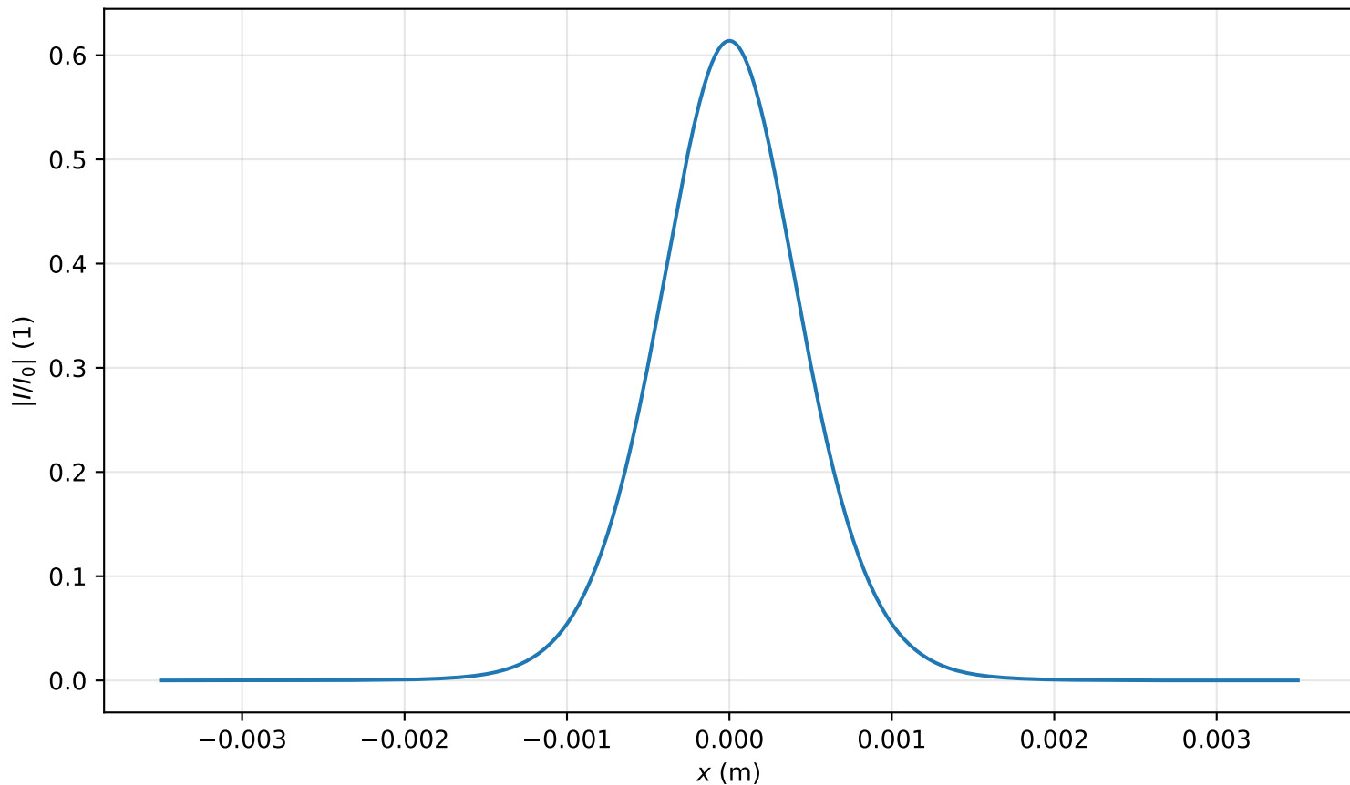
Intensity profile I(x, y = 0, z = 2.786m)/I_0 , P_{in}=0.5P_{cr} , artificial time
